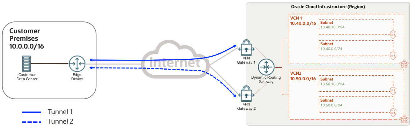
Figure 9: Site-to-Site VPN for the Same Region with Multiple VCNs with a Single Customer Edge Device
